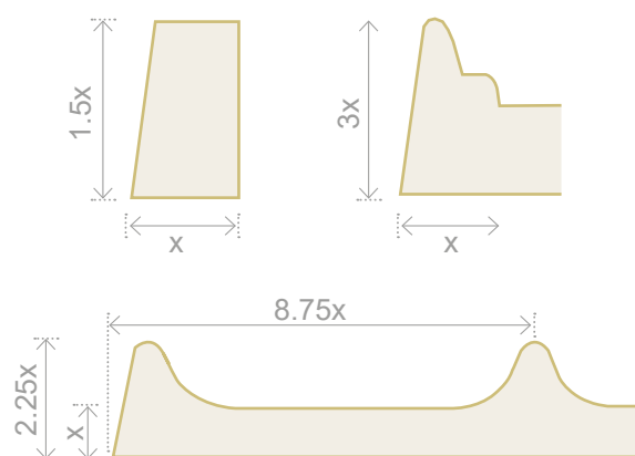
FIG. 41 Traditional parapet elements
