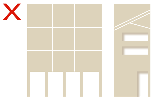
FIG. 37 Large openings at base, thin columns, blank, non-integral facades, facades not respecting privacy, should be avoided
